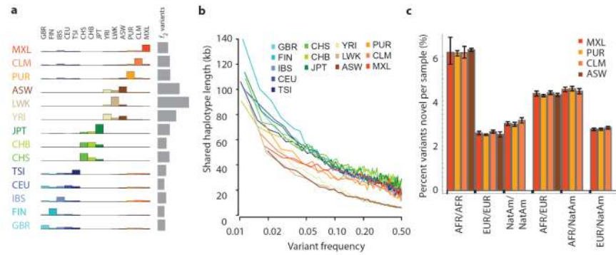
Figure 4. Purifying selection within and between populations
